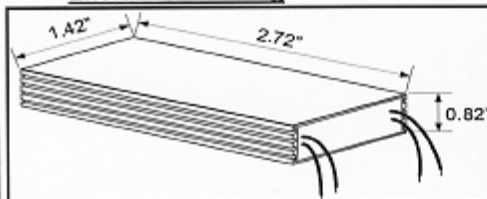
Enclosure Drawing
